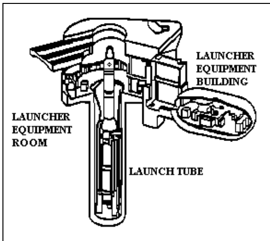
Fig. 17-4. Minuteman Launch Facility (LF)
