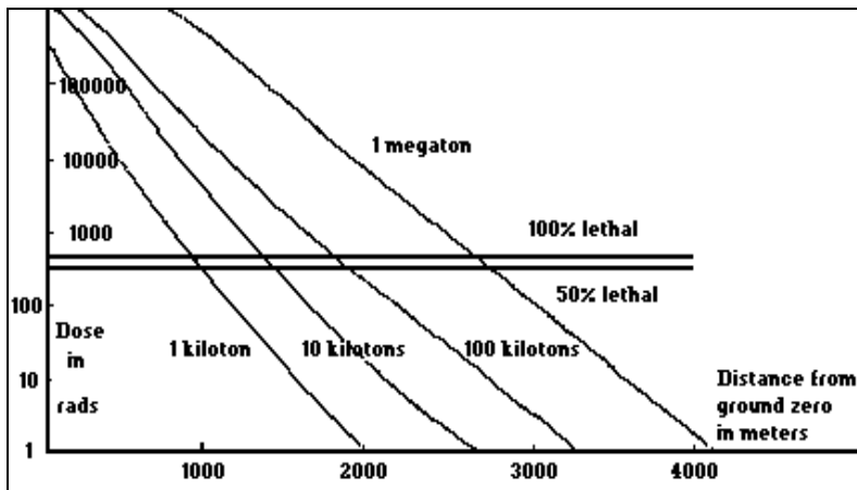
Fig. 17-3. Nuclear Weapon Effects versus Distance
