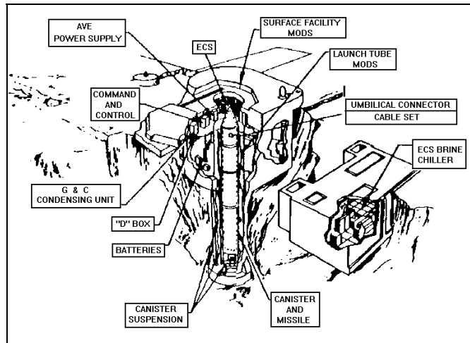
Fig. 17-6. Peacekeeper Launch Facility
