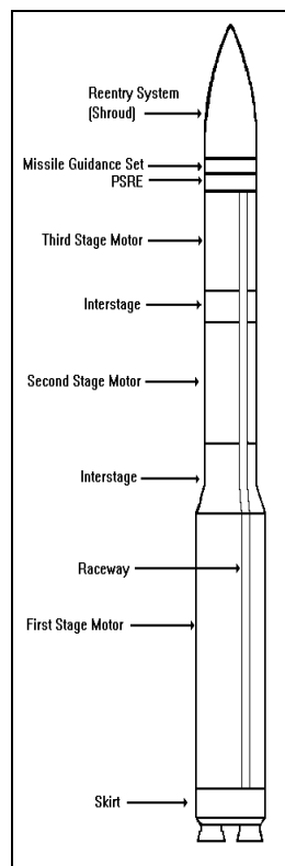
Fig. 17-5. Minuteman
