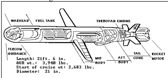
Fig. 17-10. Sea Launched Cruise Missile (SLCM)
