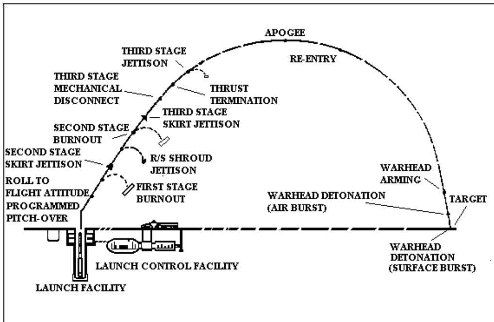
Fig. 17-2. Typical ICBM Flight Profile
